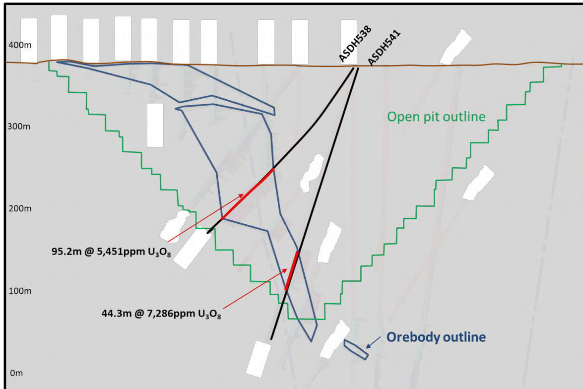
Figure 1. Section 1900NW, looking West
