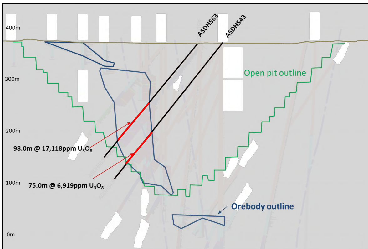
Figure 2. Section 1950NW, looking West
